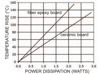
POWER DERATING
